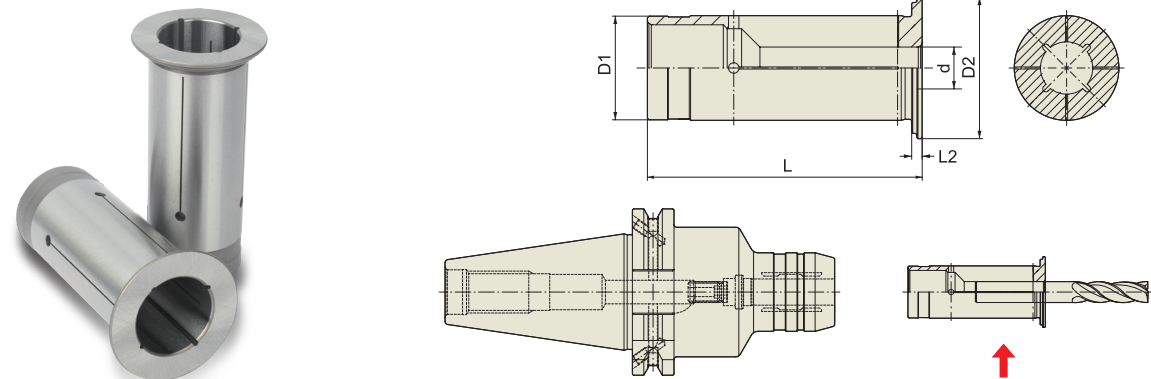
Hydraulic Chuck Collet
